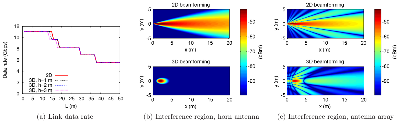
Figure 2: Key properties of 3D Beamforming. (a) Data rate vs link distance L . (b)-(c) 2D and 3D beamforming signal maps using both horn antenna and antenna arrays. The transmitter is at (0\text{m},0\text{m}) and the receiver is at (2\text{m},0\text{m}) .
